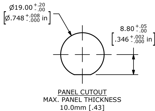
PANEL CUTOUT
