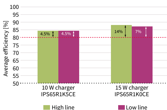
CoolMOS™ CE meets the standard efficiency requirements in charger application
