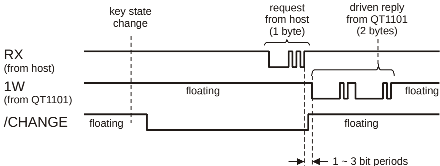
Figure 2.4 2W Operation
