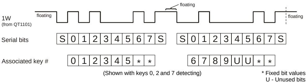
Figure 2.3 UART Response Pattern on 1W Pin
