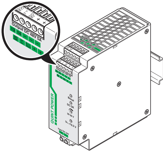
Figure 12 Signal outputs
