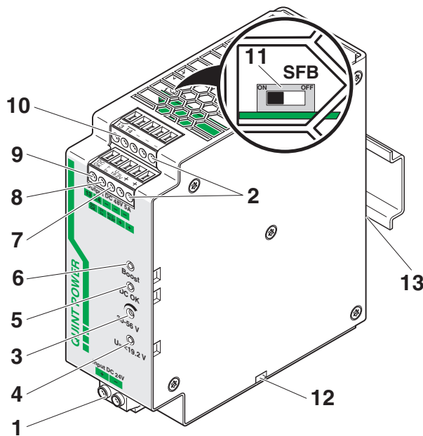
Figure 2 Function elements
