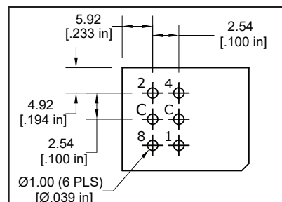
RT ANGLE R2 PCB LAYOUT
