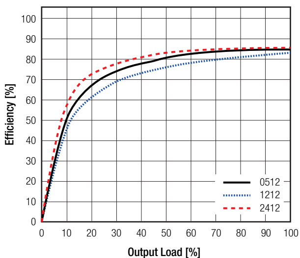
RJZ-xx12S
