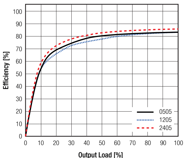
RJZ-xx05S
