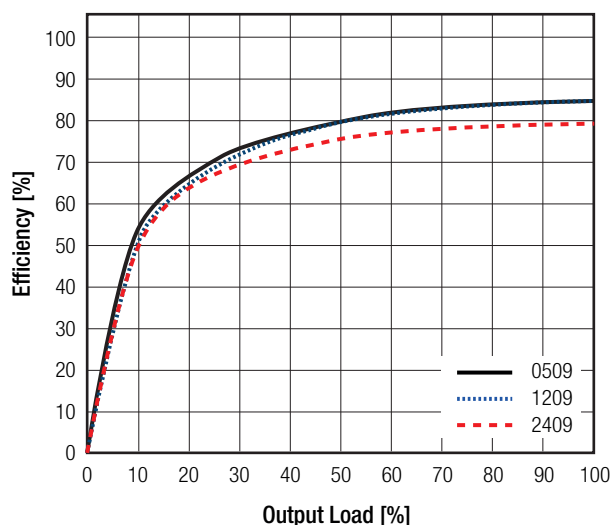
RJZ-xx09S
