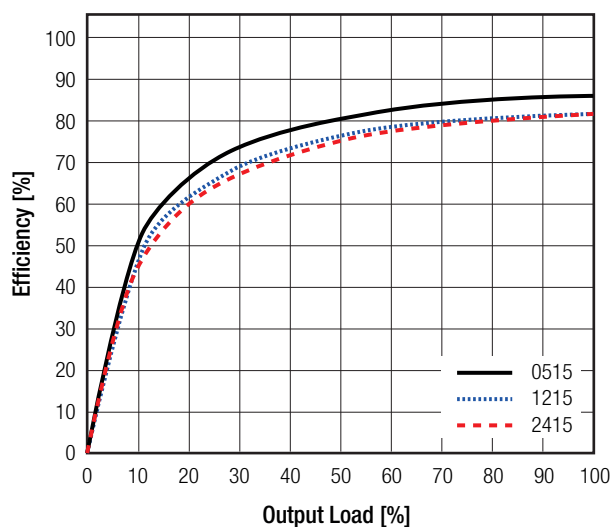
RJZ-xx15S
