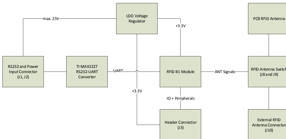
Figure 1-1 System Diagram
