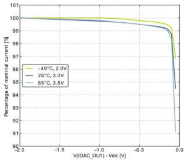
Figure 2-1 Source Current
