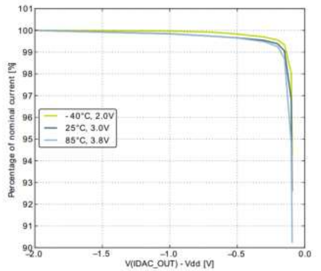
Figure 2-1 Source Current
