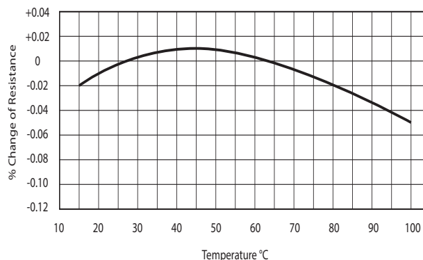
Manganin Temperature Coefficient of Resistance ±15 PPM/°C
