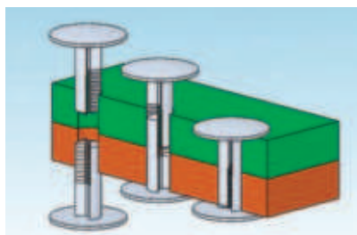
Barbed Rivet
