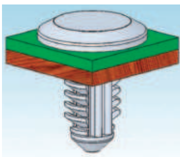
BPF Barbed Push Fastener
