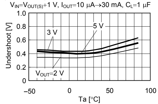
Temperature dependencies of undershoot
