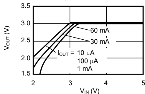
S-814A30A (Ta = 25°C)
