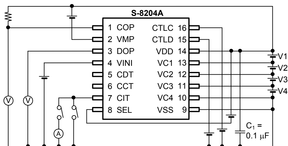
Figure 5 Test Circuit 2
