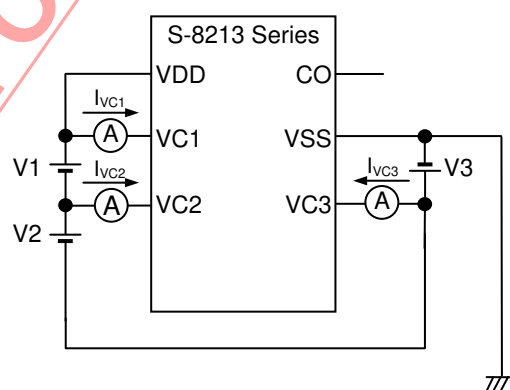
Figure 9 Test Circuit 4
