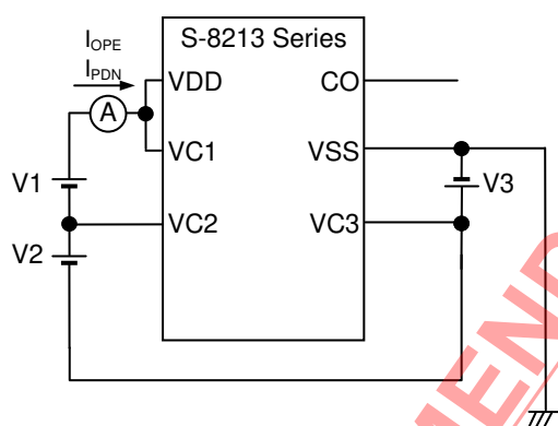
Figure 8 Test Circuit 3
