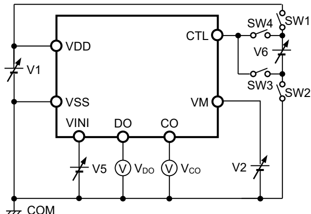
Figure 4 Test Circuit 2
