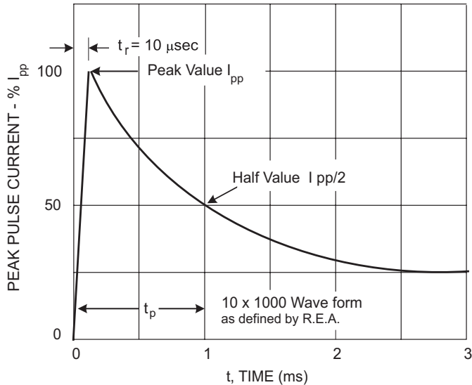
Fig. 1, Pulse Waveform
