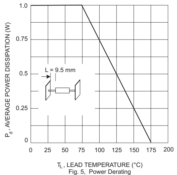
Fig. 5, Power Derating
