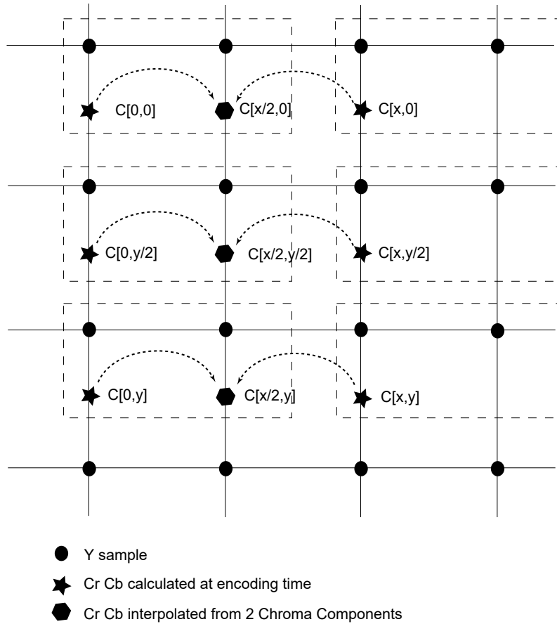
Figure 38-3. 4:2:2 Upsampling Algorithm
