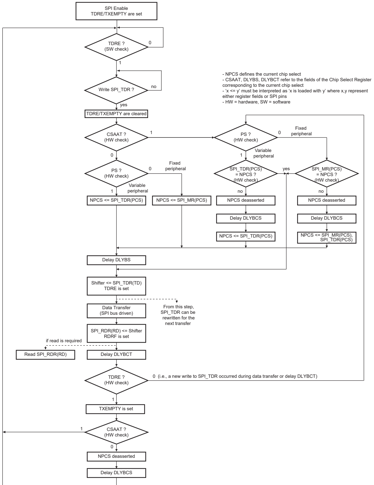
Figure 48-7. Host Mode Flow Diagram
