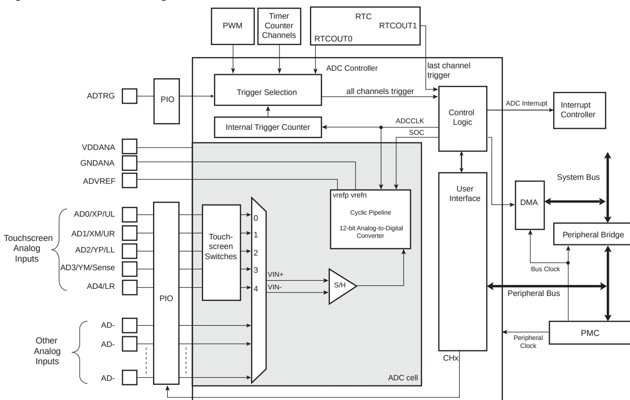
Figure 65-1. ADC Block Diagram
