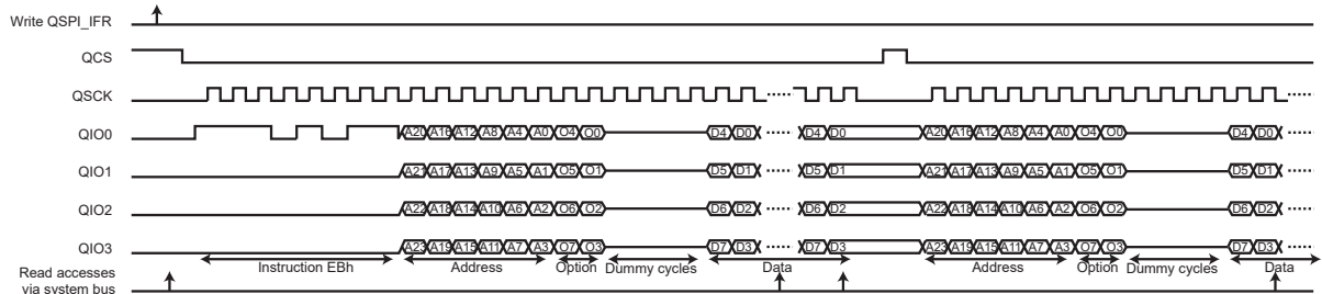
Figure 49-17. Instruction Transmission Waveform 7
