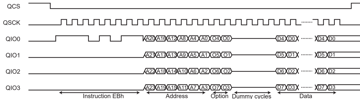
Figure 49-8. Instruction Frame
