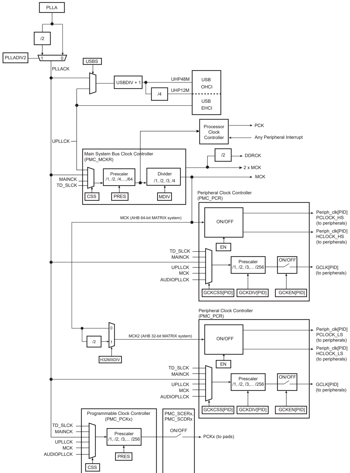
Figure 32-1. General Clock Block Diagram
