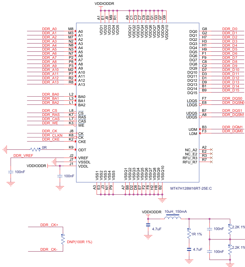
Figure 34-3. 16-bit DDR2 Hardware Configuration
