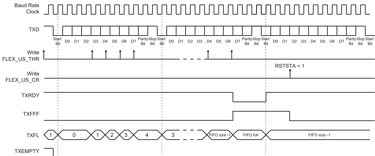
Figure 46-63. TXRDY Behavior for Single Data Access and TXRDYM = 0
