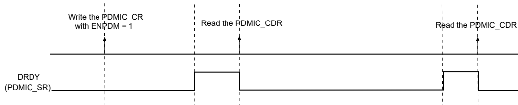
Figure 54-10. DRDY Flag Behavior
