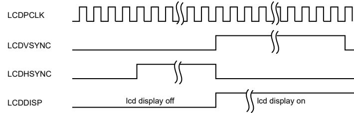
Figure 38-19. DISP Signal Timing Diagram
