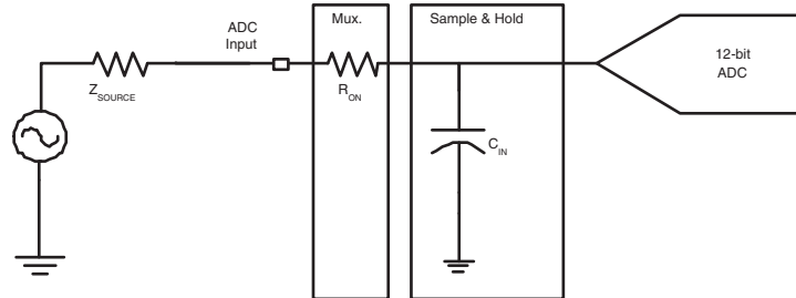
Figure 66-8. Simplified Acquisition Path
