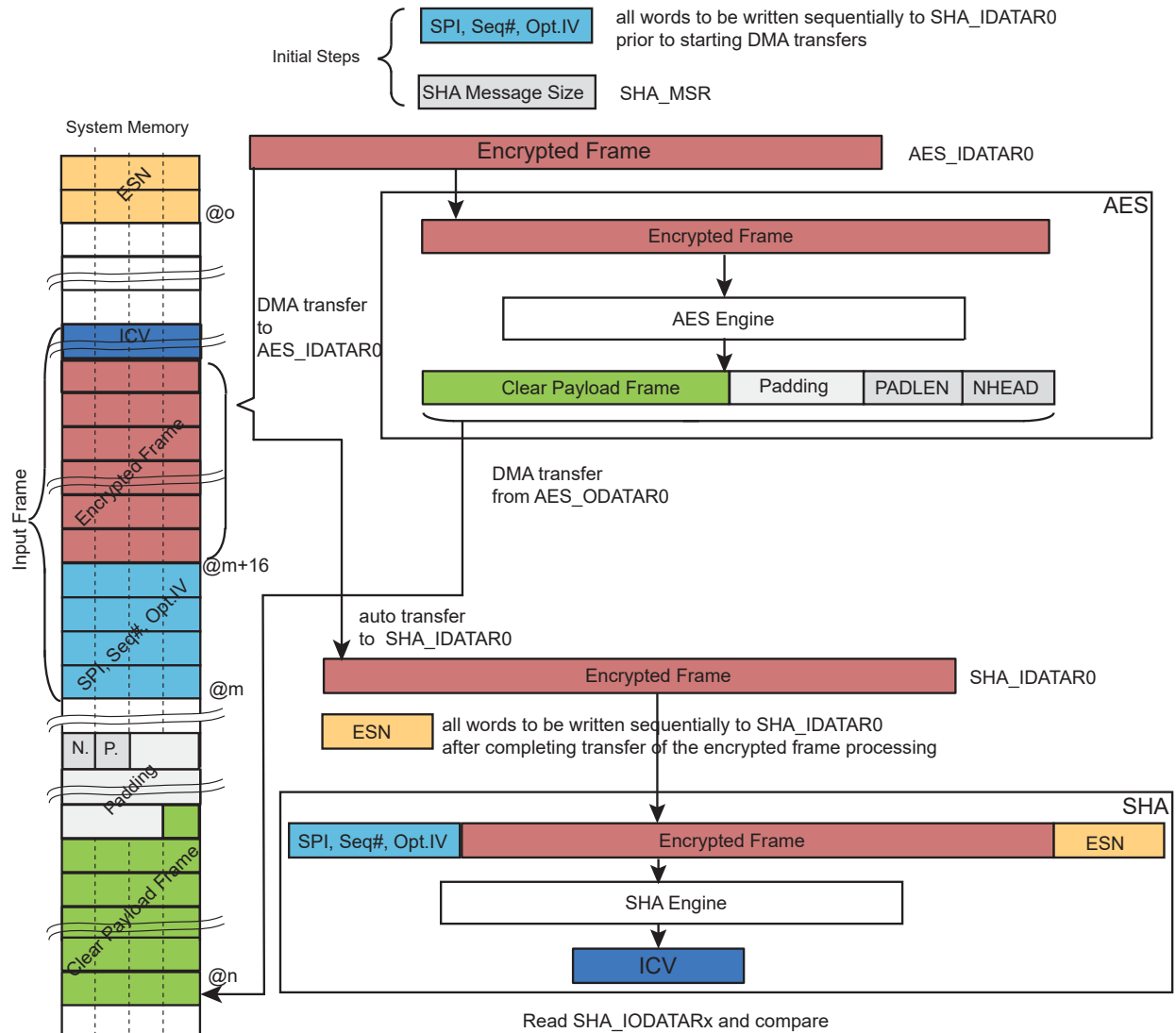
Figure 59-16. Decryption of an ESP IPsec Frame with ESN
