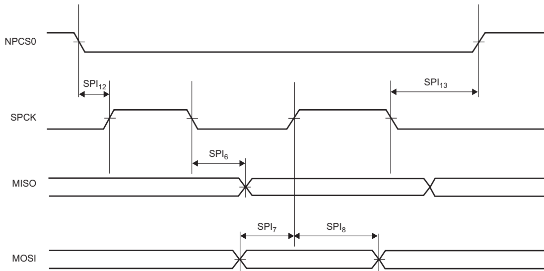
Figure 66-14. FLEXCOM in SPI Client Modes 0 and 3
