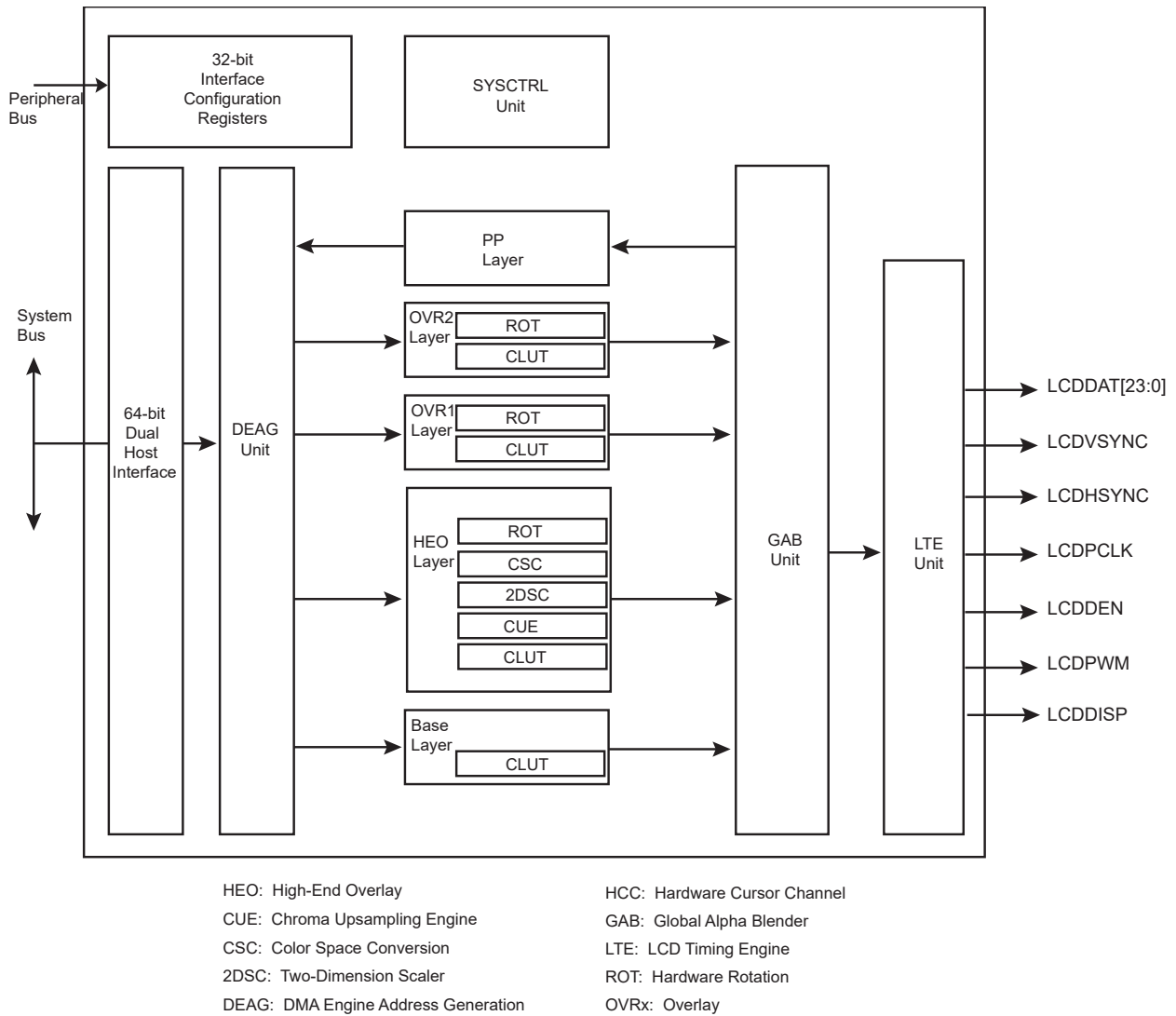
Figure 38-1. LCDC Block Diagram
