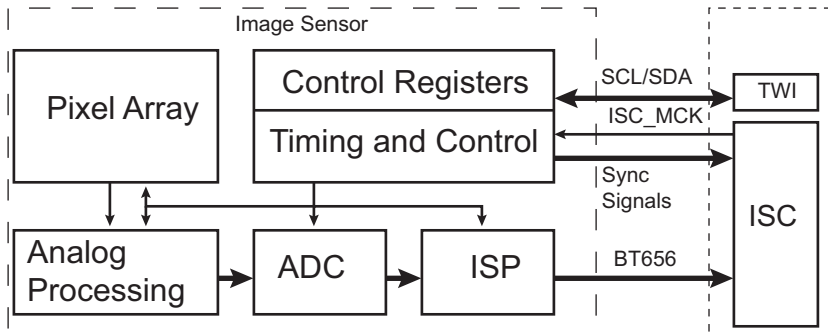
Figure 51-6. BT656 Video Interface Sensor
