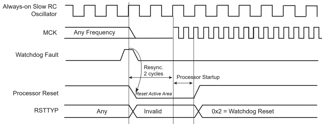
Figure 23-7. Watchdog Reset
