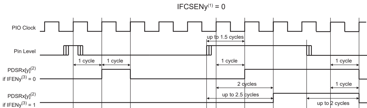
Figure 33-5. Input Debouncing Filter Timing
