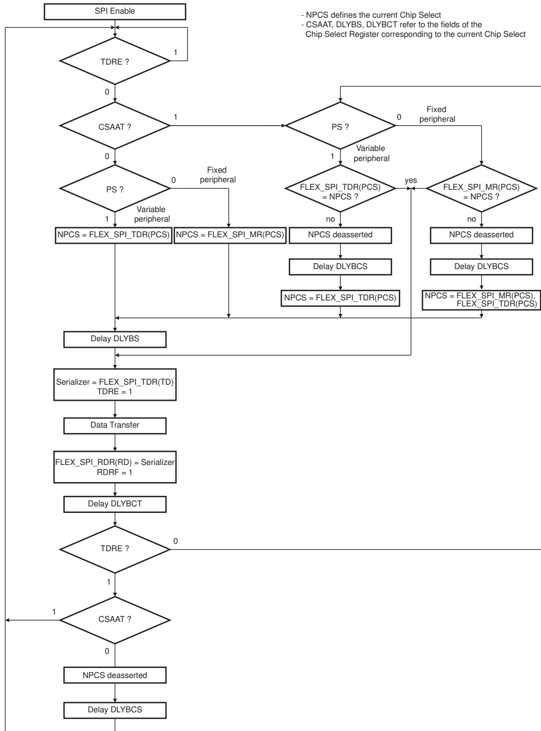
Figure 46-69. Host Mode
