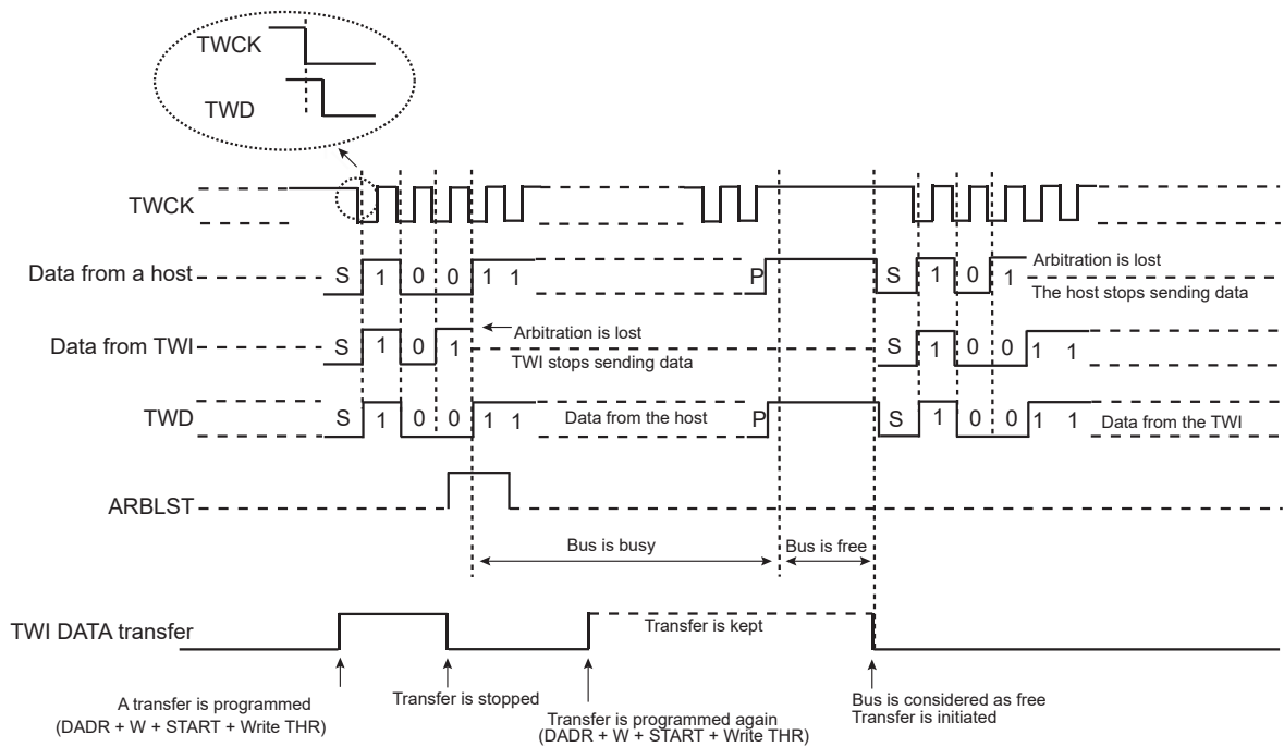
Figure 46-111. Arbitration Cases
