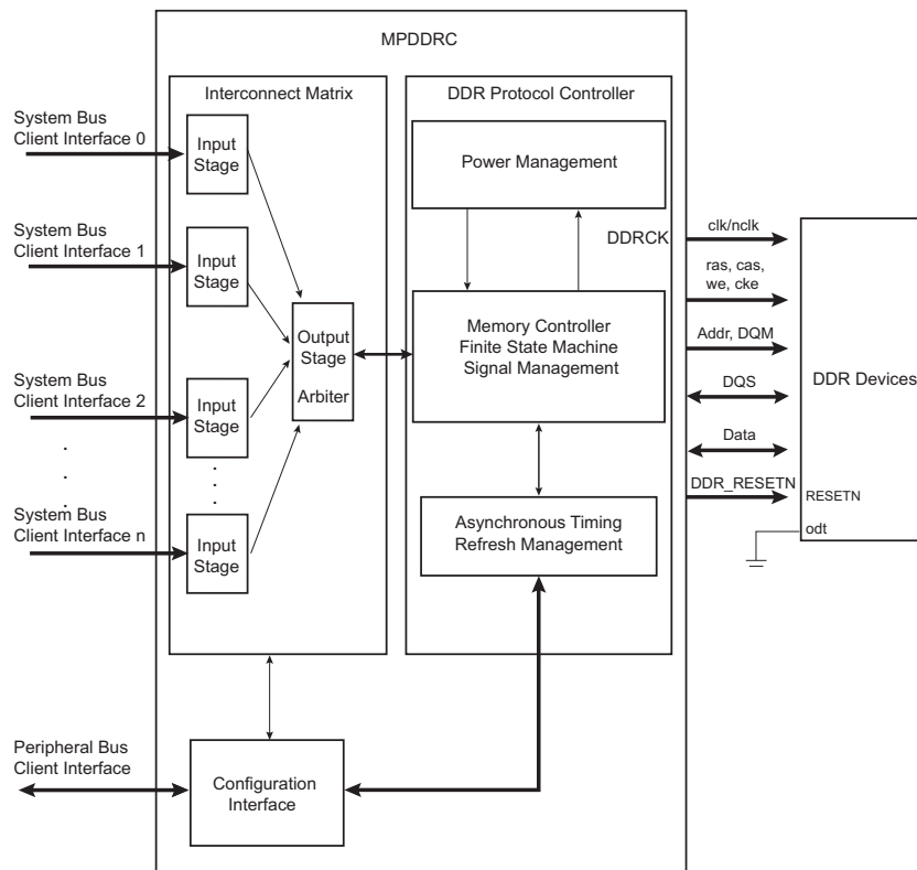
Figure 35-1. Block Diagram
