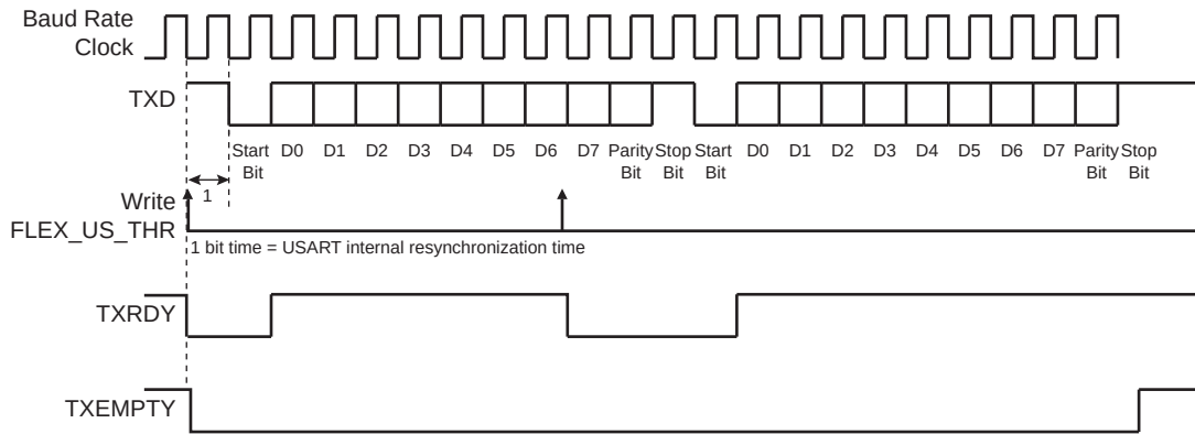
Figure 46-6. Transmitter Status
