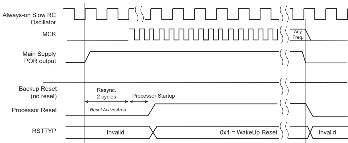
Figure 23-4. Wake-up Reset
