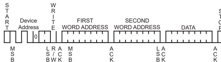
Figure 46-94. Internal Address Usage
