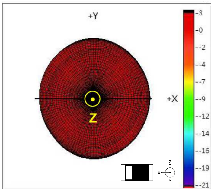
Radiation Pattern 2442MHz
