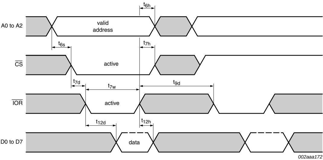
Fig 21. General read timing in 16 mode
