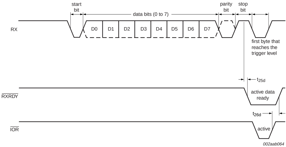
Fig 12. Receive ready timing in FIFO mode
