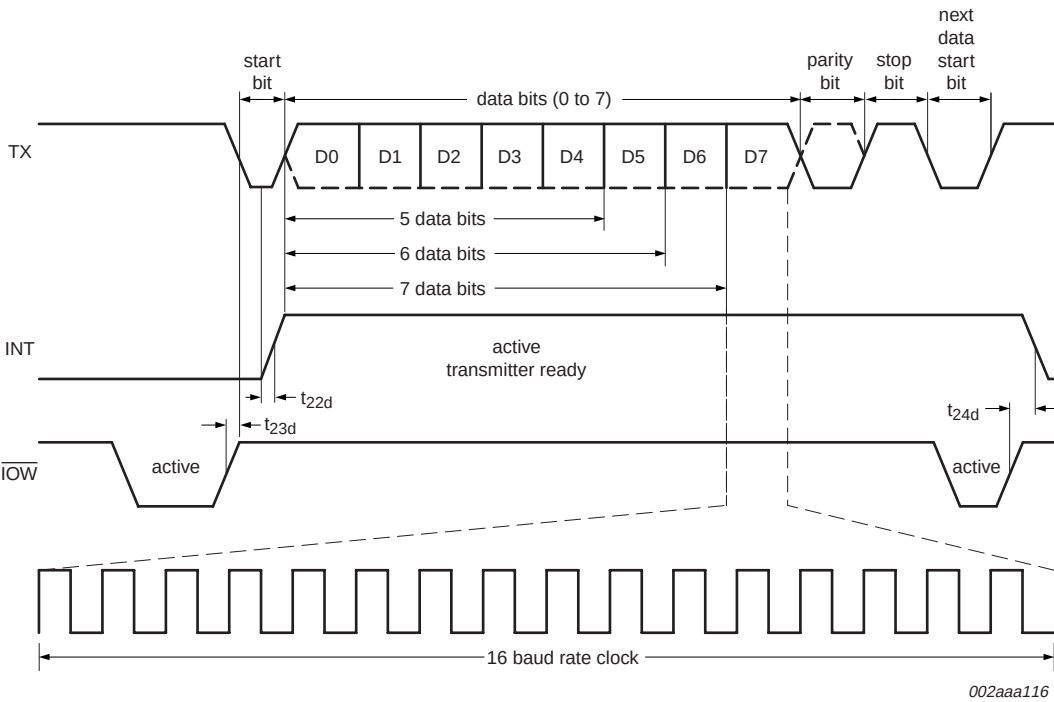
Fig 13. Transmit timing
