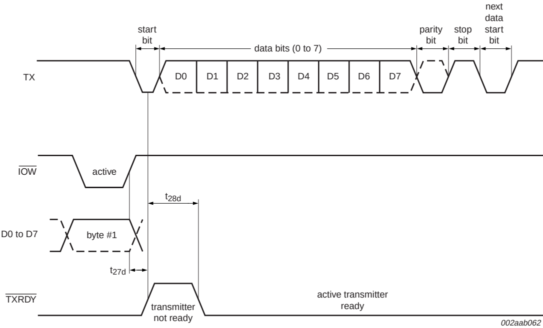
Fig 14. Transmit ready timing in non-FIFO mode
