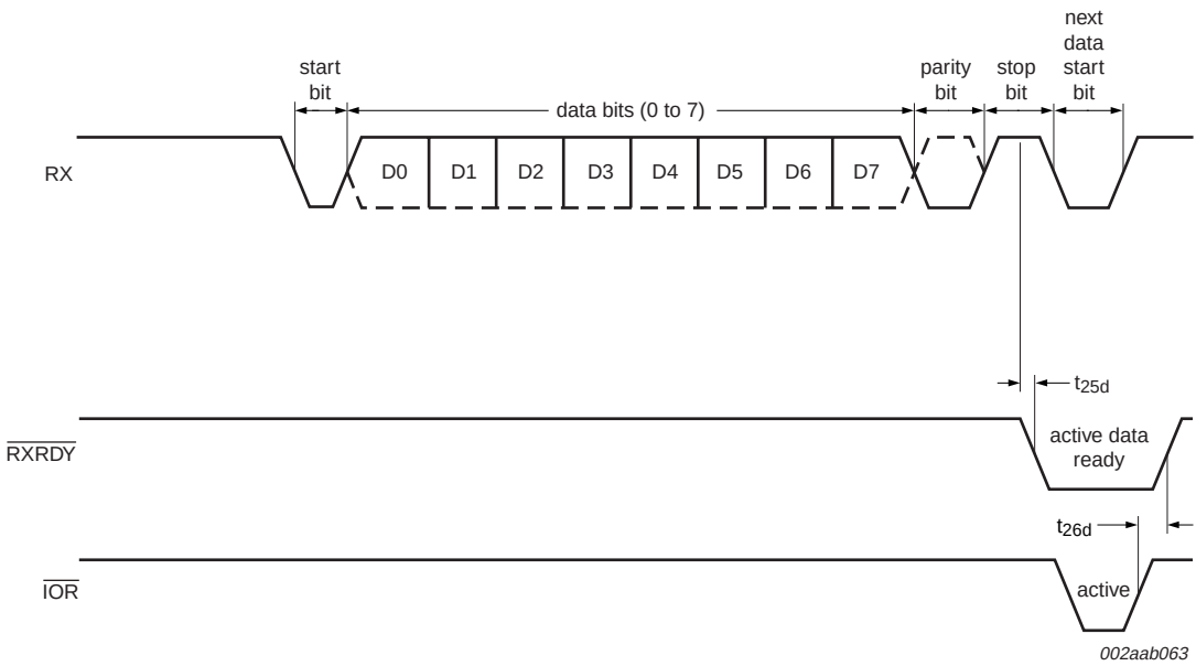
Fig 11. Receive ready timing in non-FIFO mode
