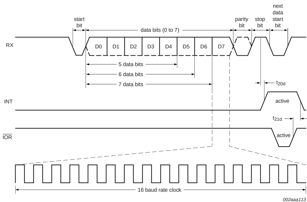
Fig 10. Receive timing
