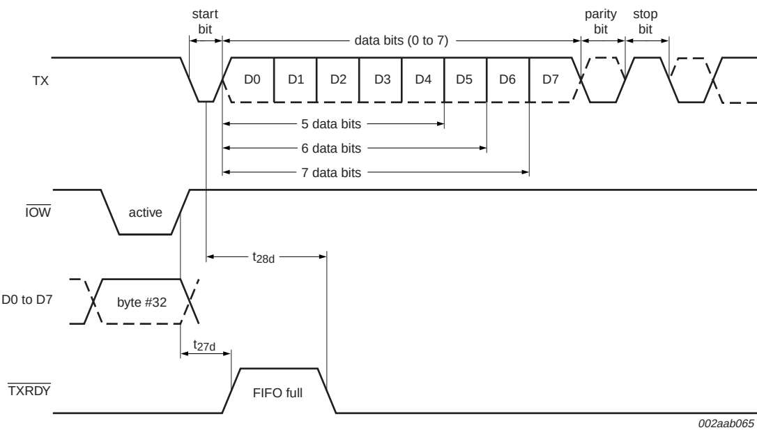
Fig 15. Transmit ready timing in FIFO mode (DMA mode '1')
