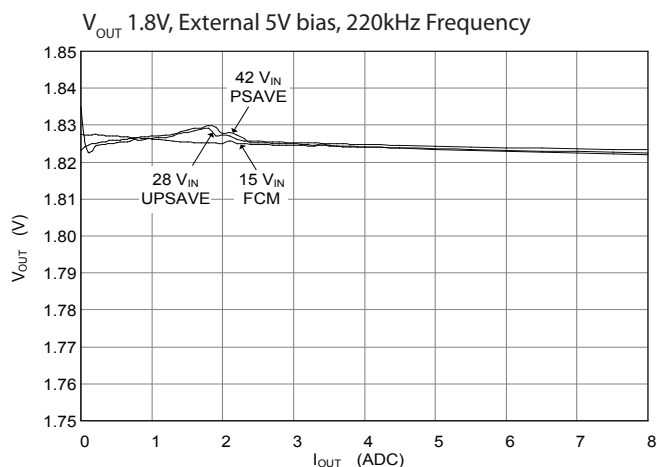
Load Regulation
