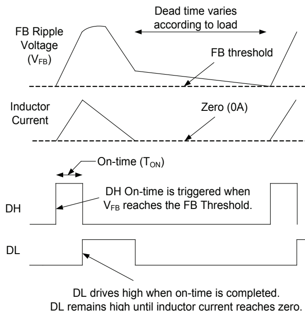
Figure 7 — Power-Save Operation
