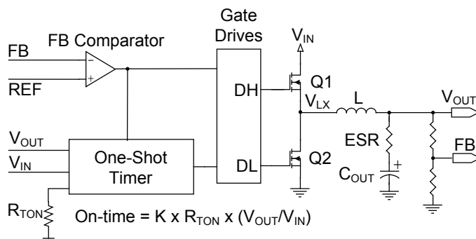
Figure 2 — On-Time Generation
