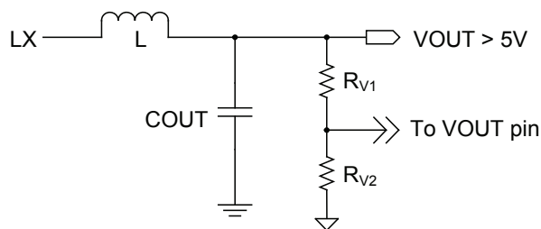
Figure 4 — Resistor Divider For V_{OUT} Exceeding 5V
