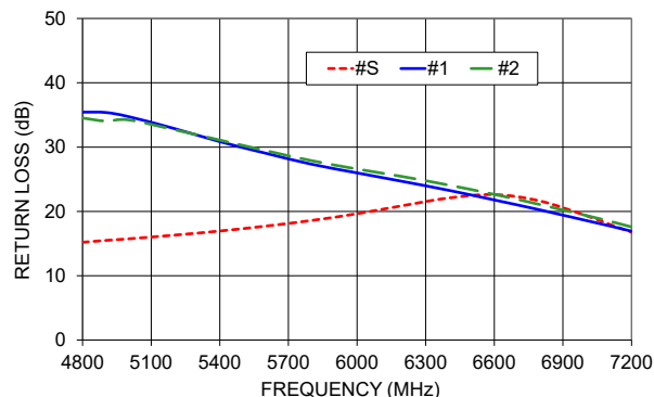
RETURN LOSS
