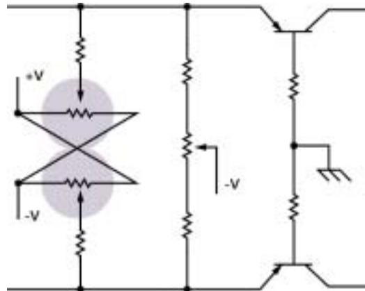
Figure 17: Trace Position Circuit
