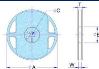
Reel Specifications
