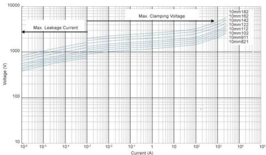
Voltage Curve - 10 mm 821K-182K
