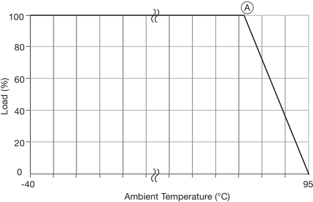
Derating curve for convection cooling
