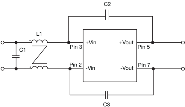
Radiated emissions
