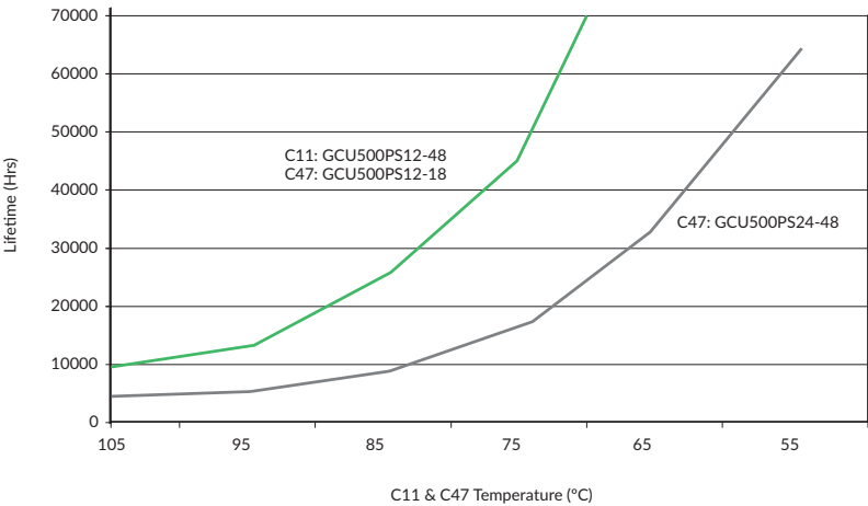
GCU500PS12-18
