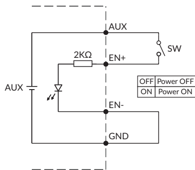
(A) Using internal 5V standby
