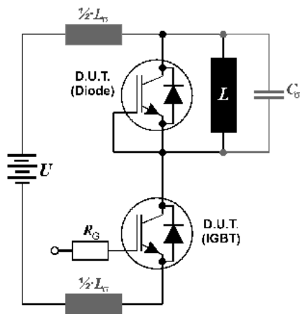
Figure E. Dynamic test circuit Leakage inductance L_\sigma = 180\text{nH} and Stray capacity C_\sigma = 900\text{pF} .
