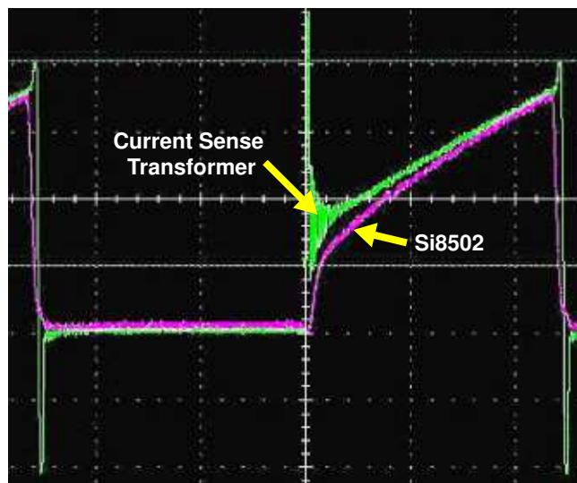
Figure 8. Leading-Edge Noise Suppression Waveforms (200 kHz, 9.3 A Load)
