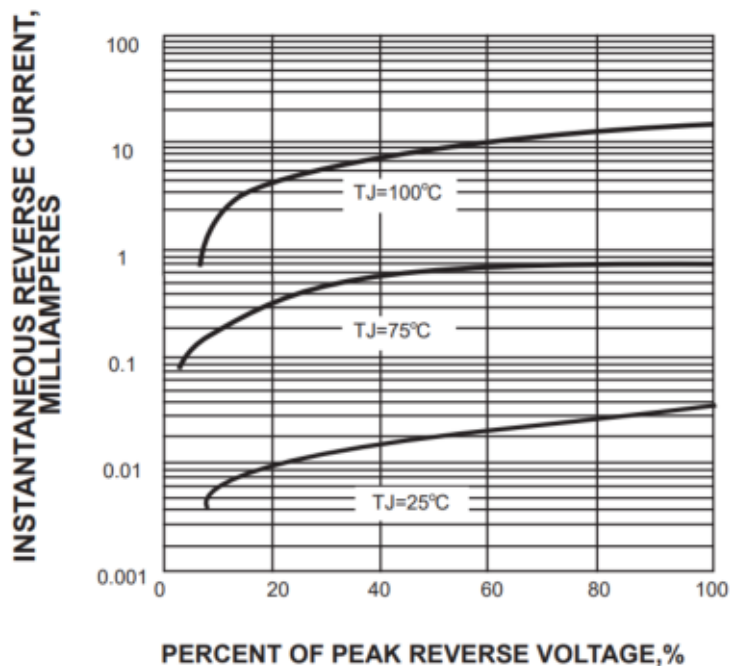
FIG. 4-TYPICAL REVERSE CHARACTERISTICS
