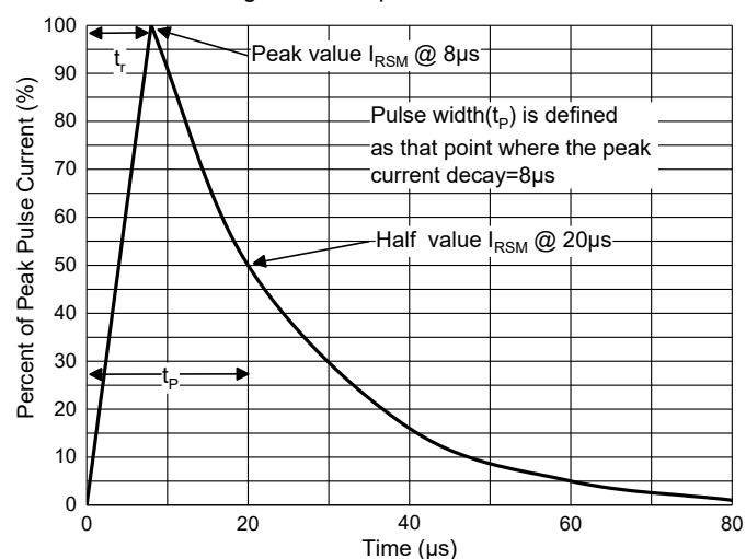
Fig. 2 - 8 X 20μs Pulse Waveform
