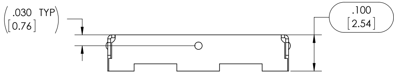
FORMED FRAME
