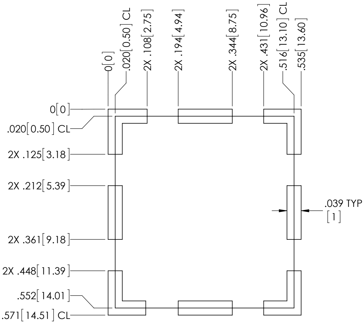
TRACE PATTERN
