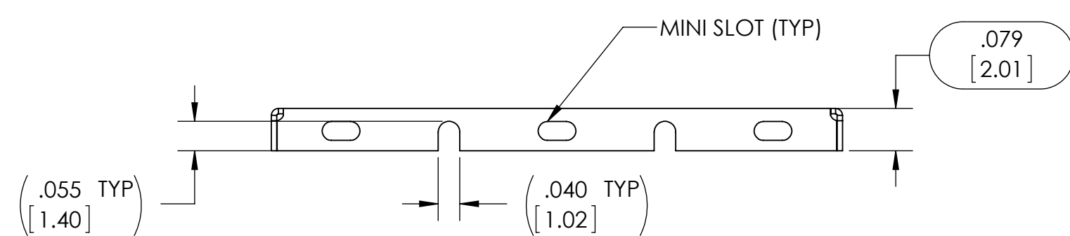
FORMED COVER
