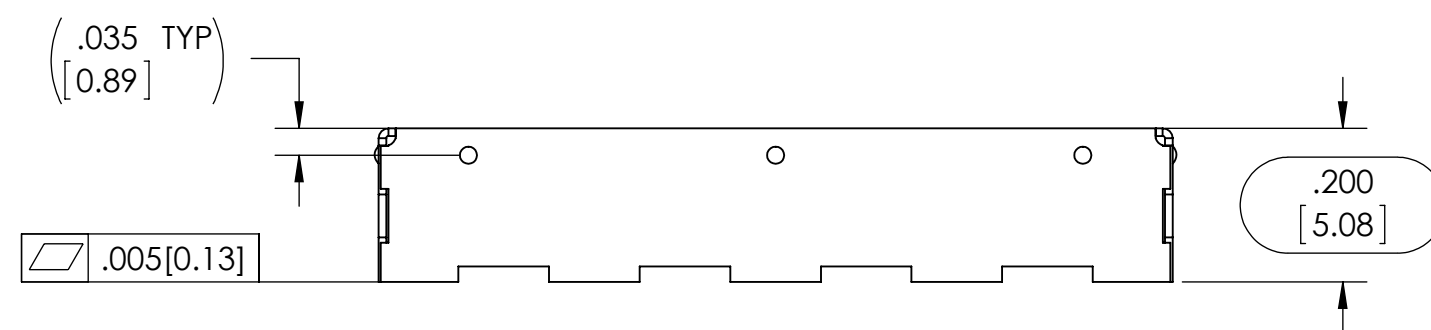
FORMED FRAME
