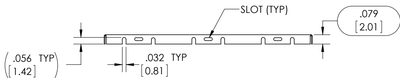
FORMED COVER
