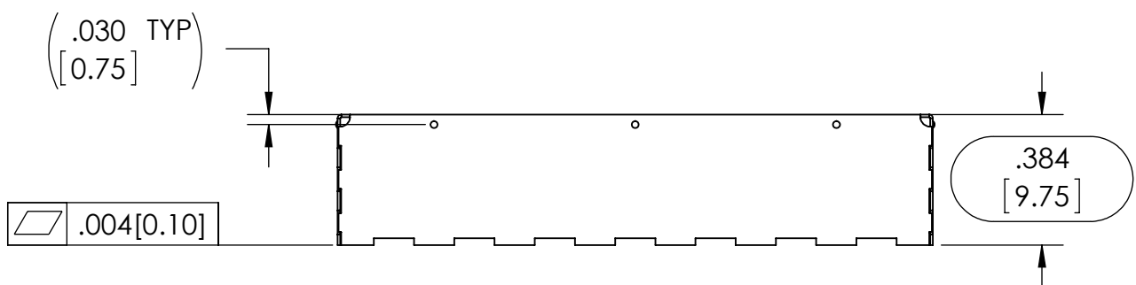
FORMED FRAME
