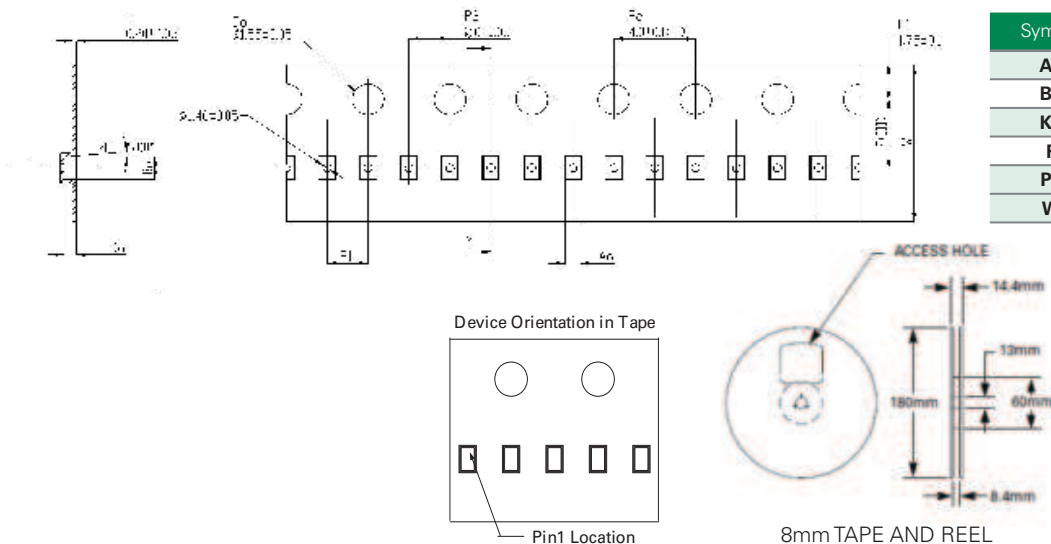
8mm TAPE AND REEL
