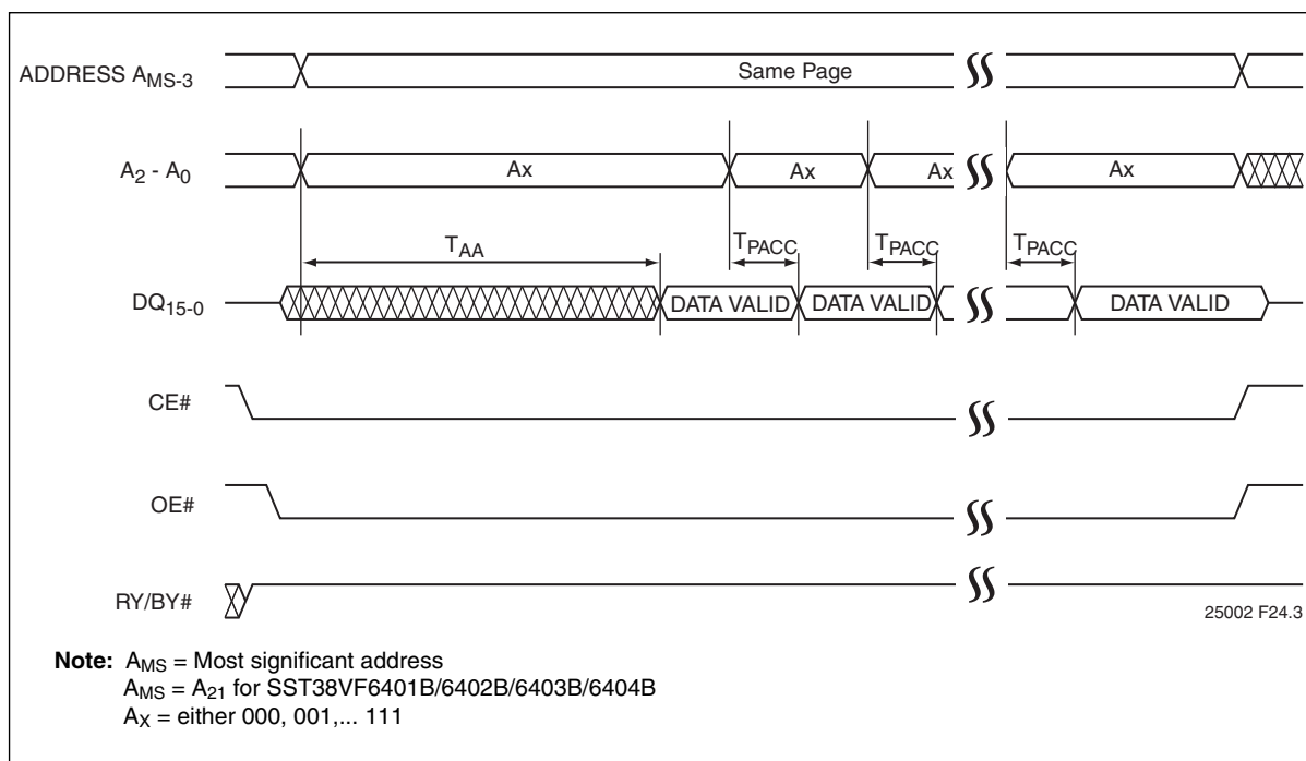
Figure 6: Page Read Timing Diagram
