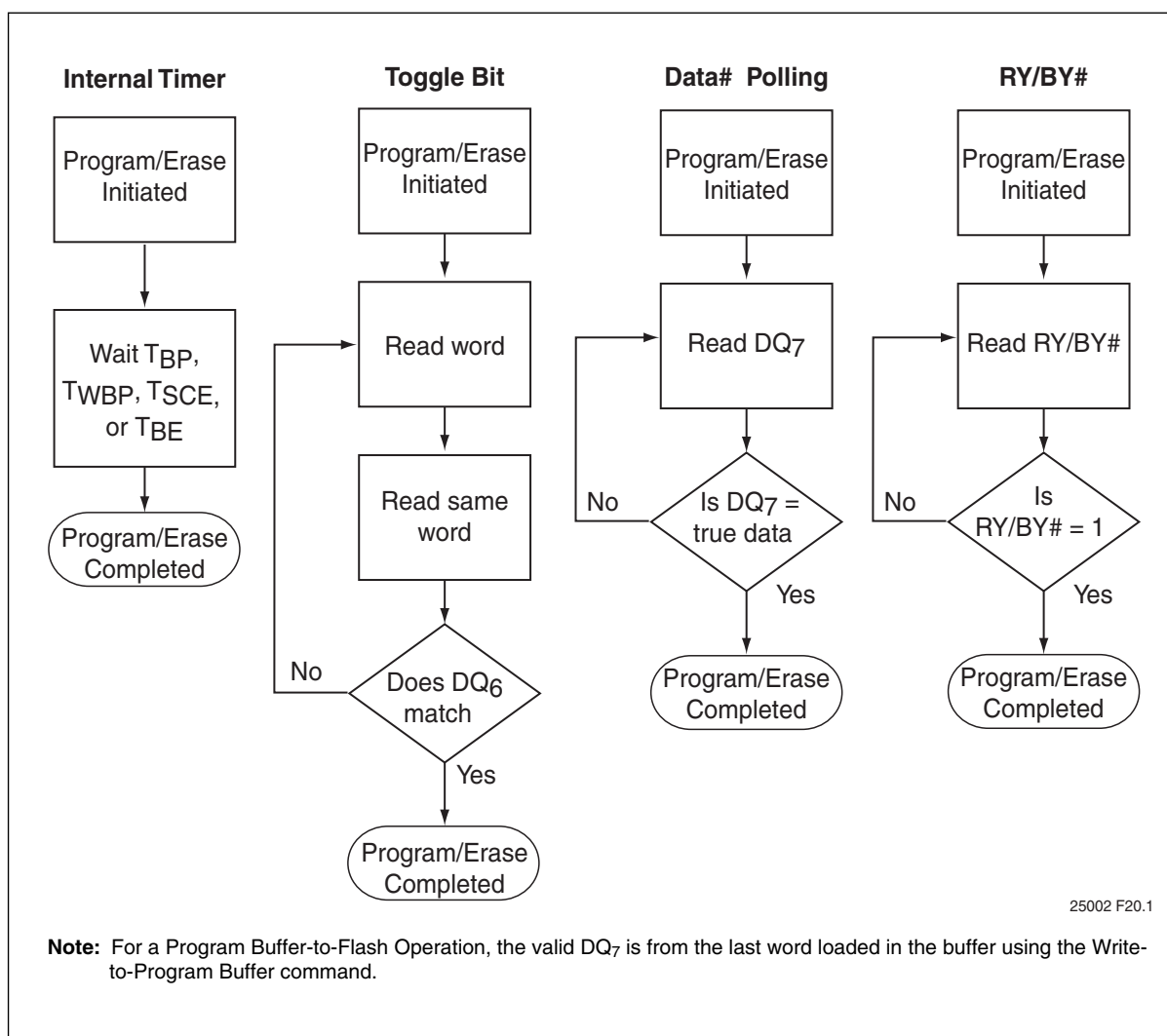
Figure 25: Wait Options
