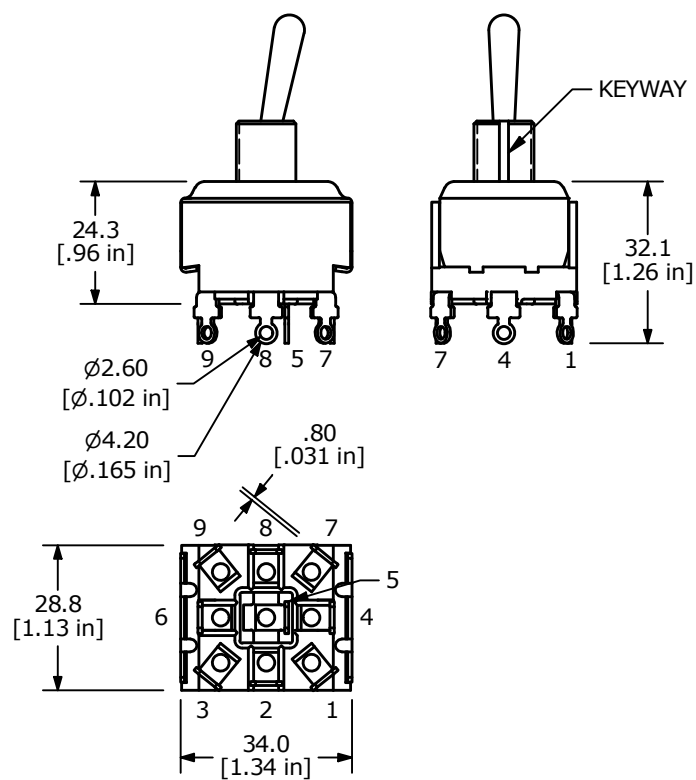
2 = SOLDER
