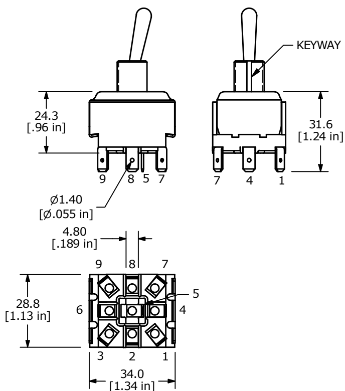
1 = 4.8mm TABS
