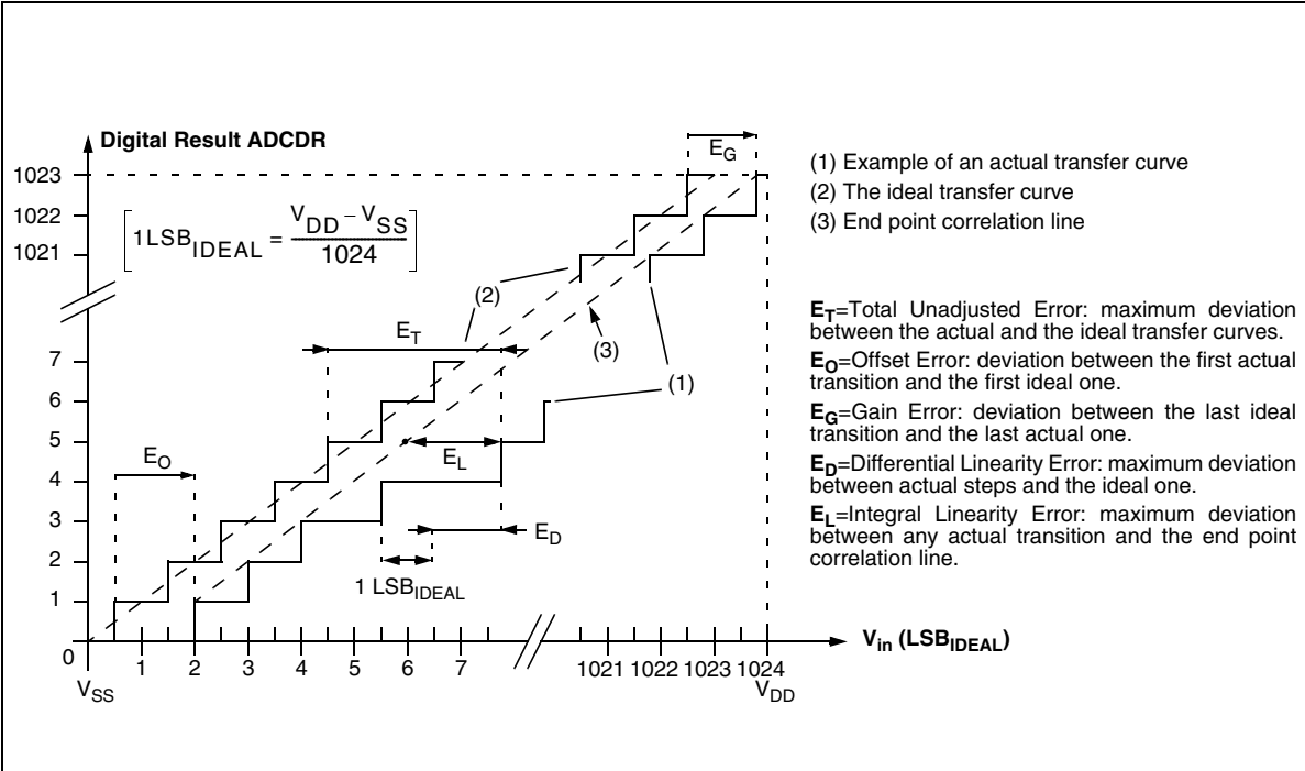
Figure 114. ADC Accuracy Characteristics
