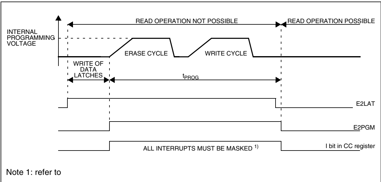
Figure 10. Data EEPROM Programming Cycle
