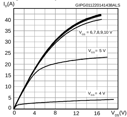
Figure 4: Output characteristics
