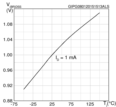
Figure 16: Normalized V_{(BR)DSS} vs temperature
