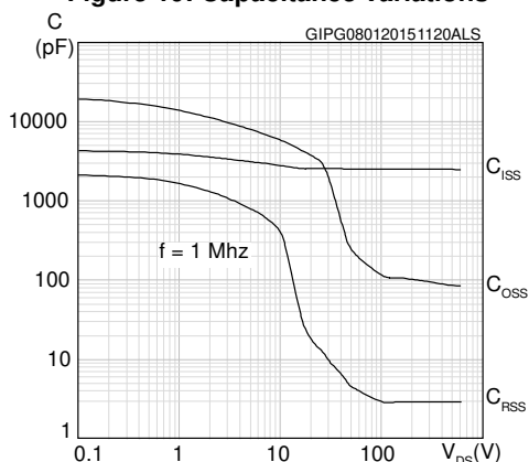
Figure 10: Capacitance variations
