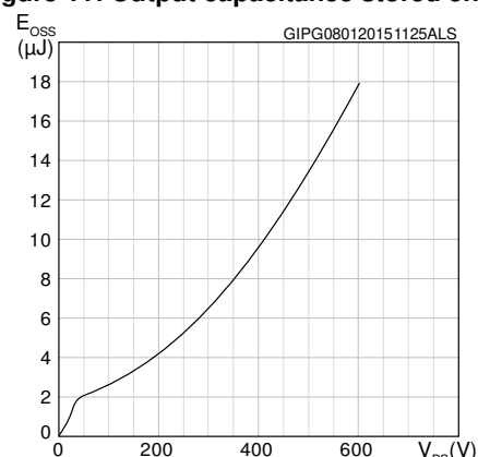
Figure 11: Output capacitance stored energy
