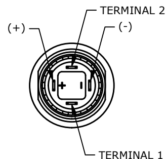
BOTTOM VIEW SHOWN WITHOUT WIRING
