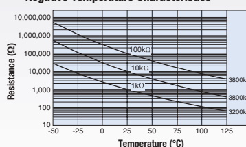
Negative Temperature Characteristics
