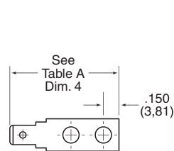
Part No. TB17
