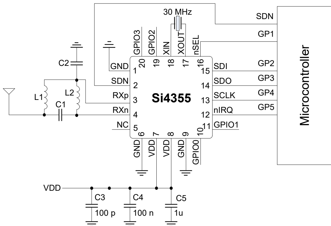
Figure 2. Si4355 Applications Circuit
