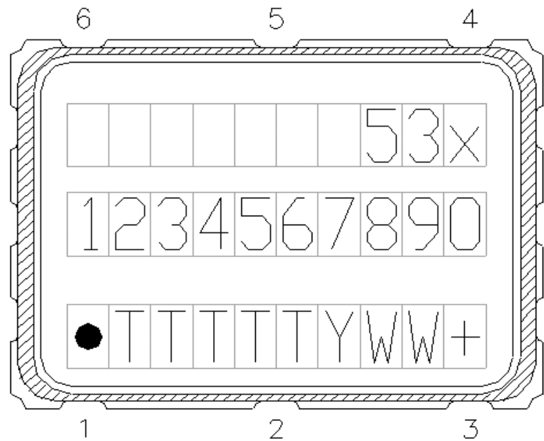
Figure 5. Mark Specification
