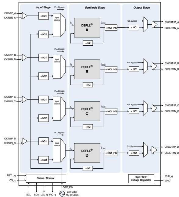
Figure 5. Functional Block Diagram
