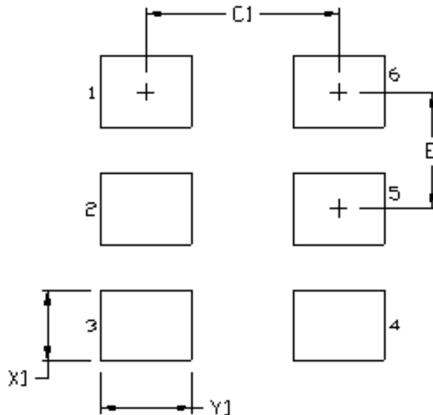
Figure 3. Si595 PCB Land Pattern Table 13. PCB Land Pattern Dimensions (mm)
