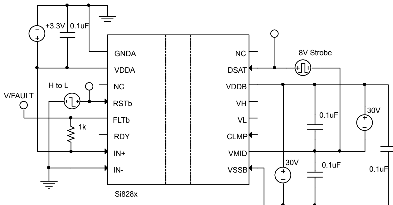
Figure 4.4. Si828x RSTb FLTb CLEAR Test Circuit
