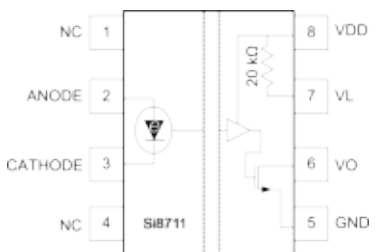
SOIC-8, DIP8 Open Collector Output with 20 kΩ Pull-up Resistor
