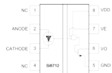
SOIC-8, DIP8 Open Collector Output with Output Enable
