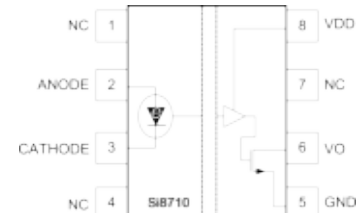
SOIC-8, DIP8 Open Collector Output
