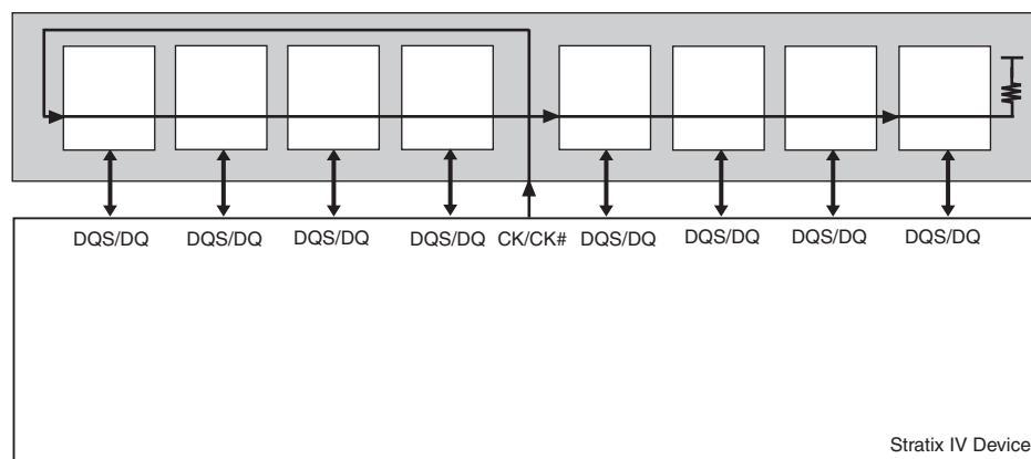
Figure 7-27. DDR3 SDRAM Unbuffered Module Clock Topology
