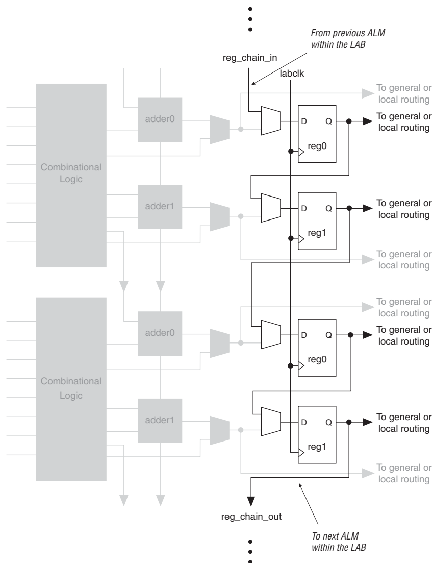
Figure 2-14. Register Chain within the LAB (1)
