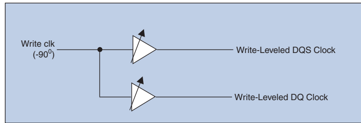
Figure 7-28. Stratix IV Write-Leveling Delay Chains and Multiplexers (1)
