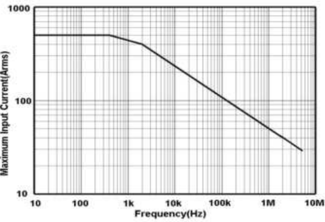
T3CP500-5 Continuous Maximum Current Input
